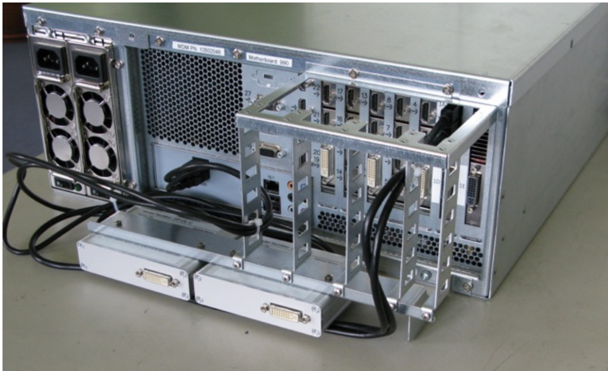
Figure 5: Rear of MDM including mounting harness
